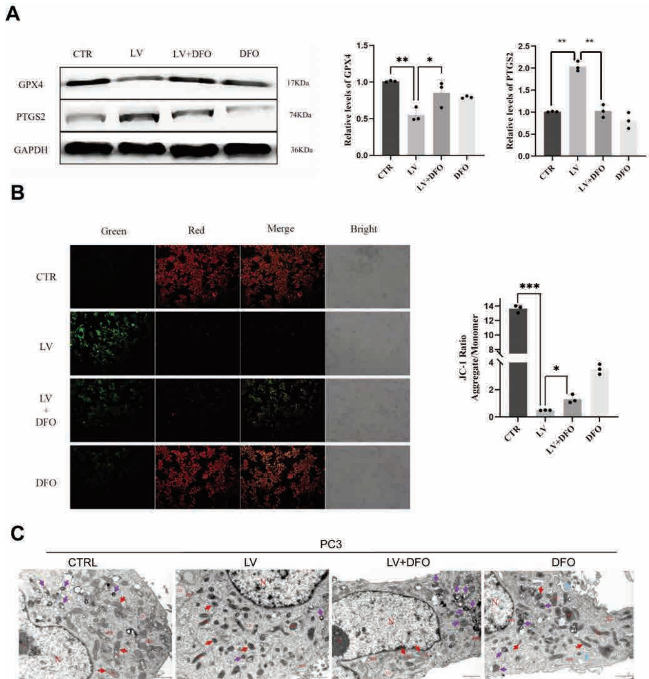
Figure 3. Combined treatment with DFO improved intracellular damage caused by lovastatin. A) Western blot showing changes in GPX4 and PTGS2 proteins; statistical analysis of GPX4 and PTGS2 protein changes was on the right. B) Image of fluorescence intensity; quantitative analysis of the ratio of red fluorescence intensity to green fluorescence intensity was on the right. C) Morphological changes in cells after co-treatment with ferroptosis inhibitors; N, nucleus; No, nucleolus; Mi, mitochondria; RER, rough endoplasmic reticulum; LD, lipid droplet; scale bar: 1 \mu m; ns, no statistically significant difference; n=3 ; * p>0.05 , ** p<0.01 ; *** p<0.001 .
