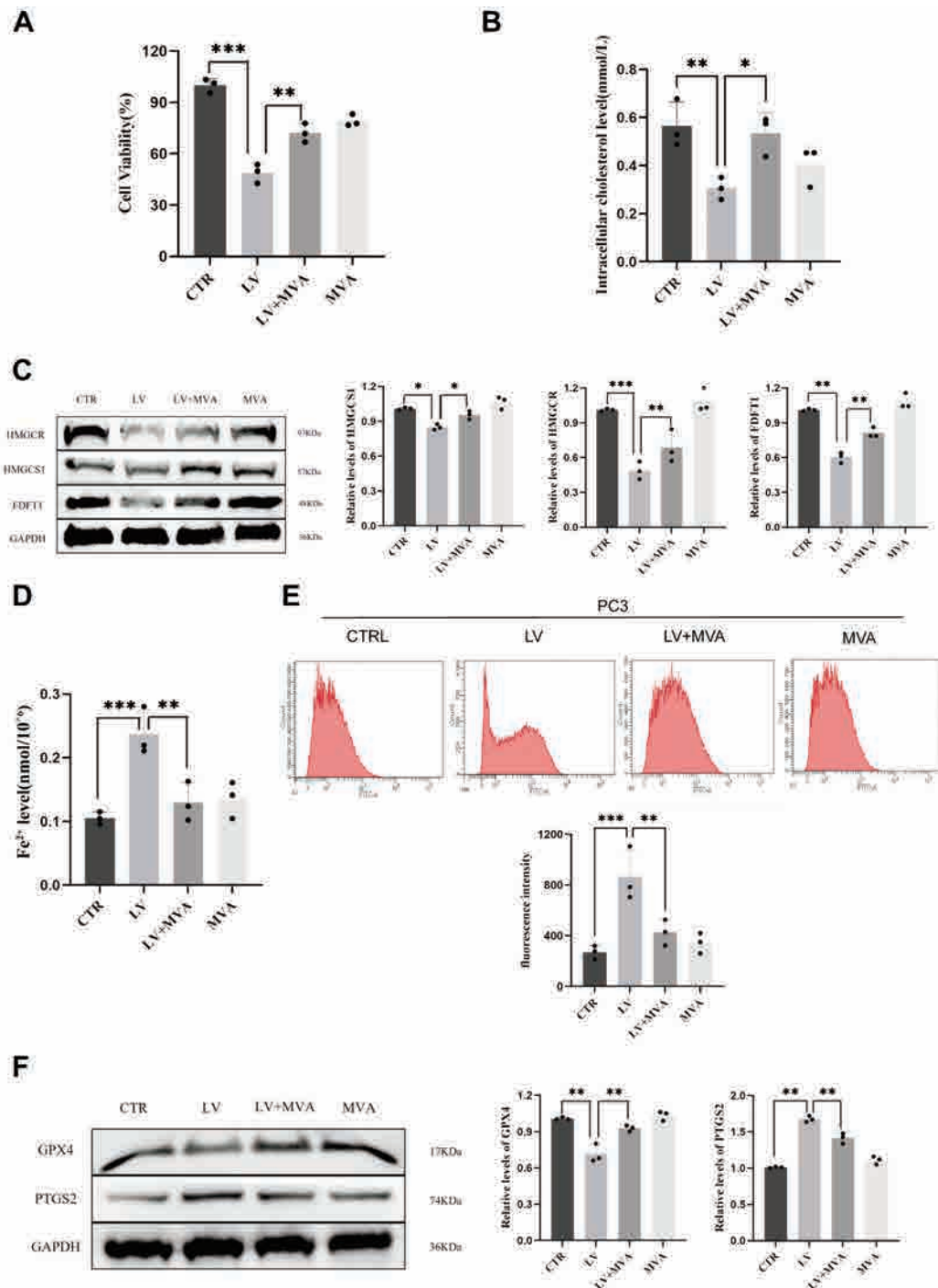
Figure 4. LV promotes ferroptosis in prostate cancer cells by inhibiting the MVA pathway. A) Survival rate of PC3 cells after treatment with lovastatin and/or MVA. B) Intracellular cholesterol level after treatment with lovastatin and/or MVA. C) Western blot of intracellular HMGCR, HMGCS1, and FDFT1 protein levels after co-treatment with MVA; quantitative analysis of HMGCR, HMGCS1, and FDFT1 protein expression levels was on the right. D) Intracellular Fe 2+ levels after co-treatment with MVA. E) Intracellular ROS levels after co-treatment with ferroptosis inhibitors; quantitative analysis of fluorescence intensity was below. F) Intracellular GPX4 and PTGS2 protein levels after co-treatment with MVA; quantitative analysis of GPX4 and PTGS2 protein expression levels. ns, no statistically significant difference; n=3; * p >0.05, ** p <0.01, *** p <0.001.
